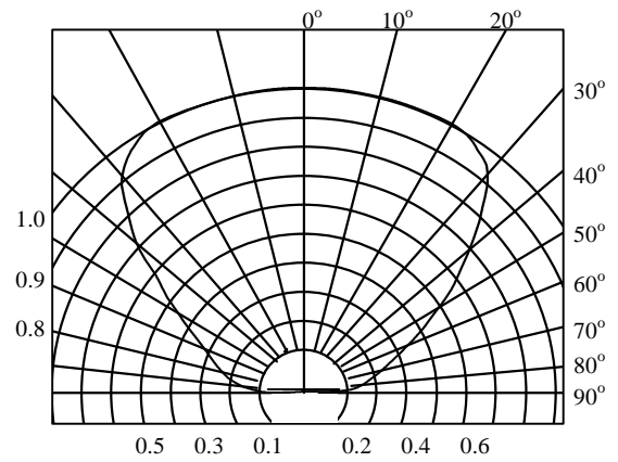
FIG.5 Radiation Characteristic I_{\text{rel}} = f(\theta)
